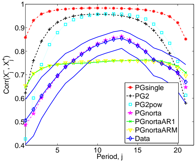
Sample correlation between past and future demand.
