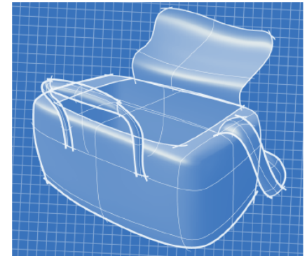
(c) Shading
