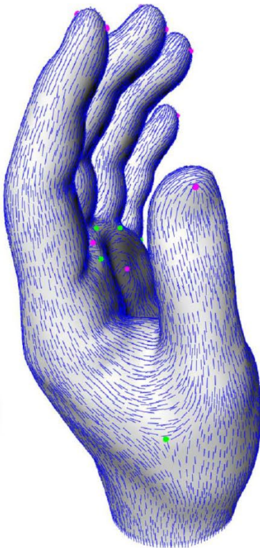
direction fields
