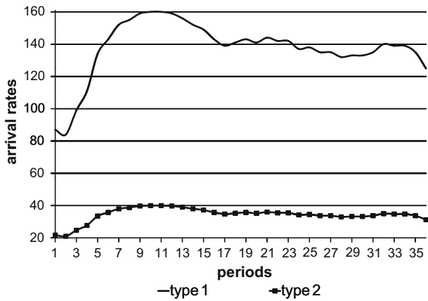
Fig. 1. Small center: arrival rates.
