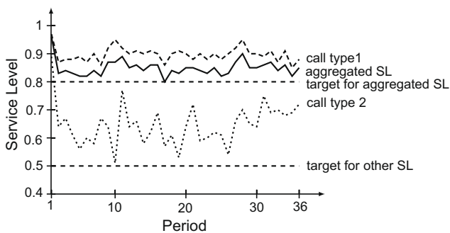
Fig. 2. Small center: service levels by period.
