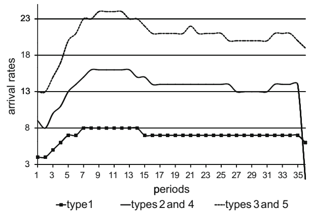
Fig. 3. Medium-sized center: arrival rates.
