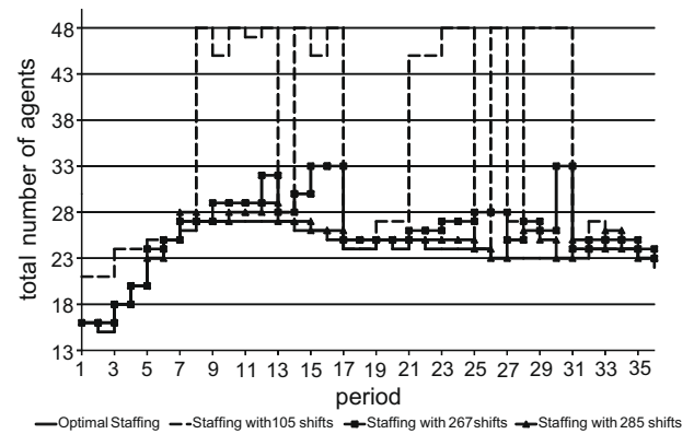
Fig. 4. Small center: staffing solutions with 105, 267 and 285 shift types.
