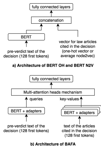
Figure 2: Architecture diagrams of BERT-OH, BERT-N2V both on part a) and BAFA on part b).
