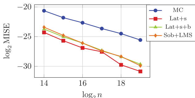
Figure 5. (Color online) MISE vs n in Log-Log Scale for the SAN Example
