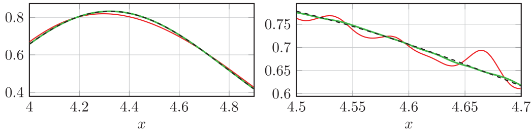
Figure 3. (Color online) The CDE Under MC (Solid Line, Red in the Color Version), Under RQMC (Light Solid Line Almost Superposed to the Dashed Line, Green in the Color Version) and the True Density (Black, Dashed) for \mathcal{G}_{-1} with n = 2^{10} (Left) and for \mathcal{G}_{-2} with n = 2^{16} (Right) for the Cantilever Example
