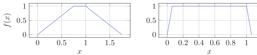
Figure 1. (Color online) Exact Density of X for the Model in Example 2 with \epsilon = 3/4 (Left) and \epsilon = 1/16 (Right)
