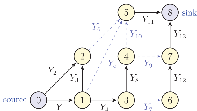
Figure 4. (Color online) A Stochastic Activity Network with the Cut \mathcal{L} = \{5, 6, 7, 9, 10\} Formed by the Dashed Arrows
