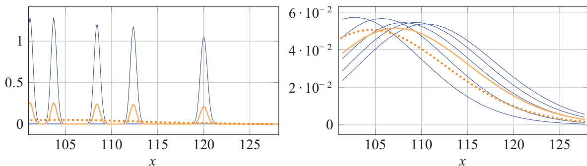
Figure 6. (Color online) Five Realizations of the Density Estimator (Light Solid Lines), Their Average (Dotted Line, Orange in the Color Version), and the True Density (Thick Black Line) for the Sequential CDE (Left) and the Bridge CDE (Right) for the Asian Option Example
