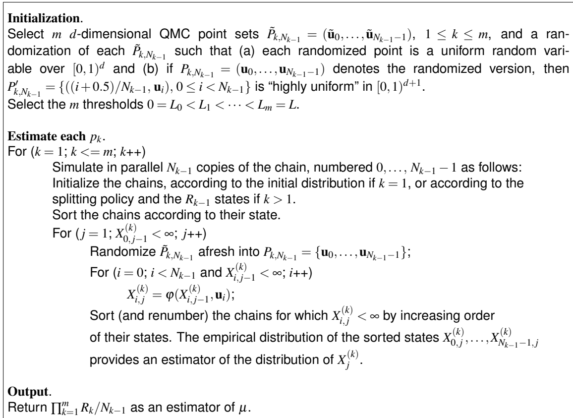
Figure 1: Combined array-RQMC/splitting algorithm
