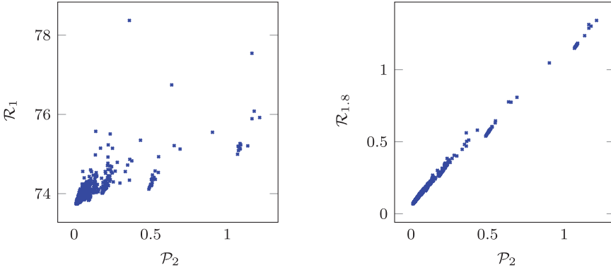
Fig. 8. Values of \mathcal{R}_\alpha against those of \mathcal{P}_2 of 1000 random lattices in dimension s = 5 with n = 2^{12} , for \alpha = 1 (left) and 1.8 (right). Note the different vertical scales.
