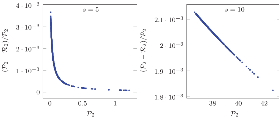
Fig. 6. Distance from \mathcal{R}_2 to \mathcal{P}_2 in units of \mathcal{P}_2 , in dimension s = 5 (left) and 10 (right), for 1000 random lattices with n = 2^{12} . Note the different vertical and horizontal scales.
