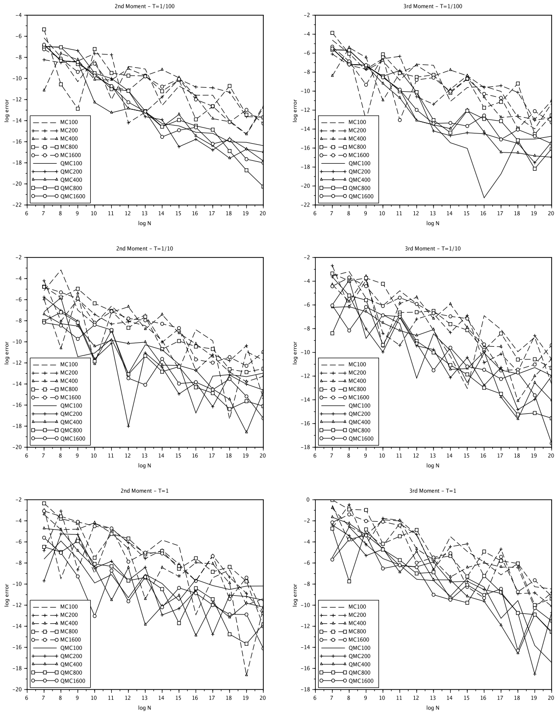
Fig. 1. Error in the second (left) and third (right) moment estimation at time 1/100 (top) 1/10 (middle) and 1 (bottom), as a function of N (number of particles varying from 2^7 to 2^{20} ), for P (number of time steps) between 100 and 1600. Log–log plots of the MC (dashed line) versus QMC (solid lines) results.
