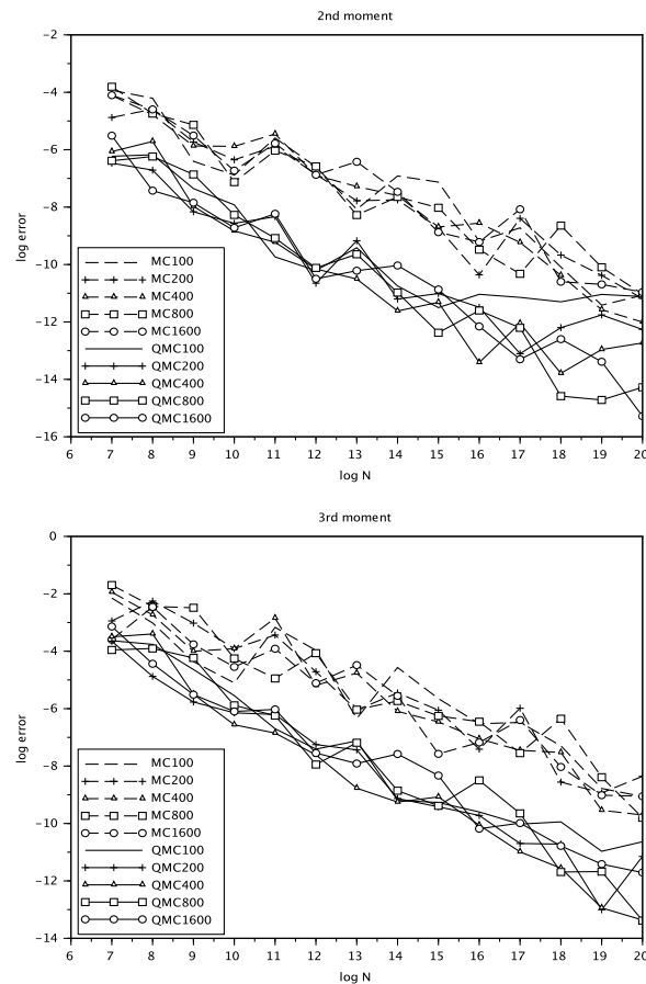
Fig. 2. Mean error in the second (top) and third (bottom) moment estimation as a function of N (number of particles varying from 2^7 to 2^{20} ), for P (number of time steps) between 100 and 1600. Log–log plots of the MC (dashed line) versus QMC (solid lines) results.
