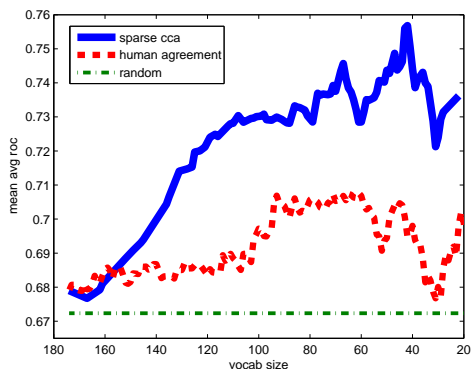
Figure 1: Comparison of vocabulary selection techniques: We compare retrieval performance using vocabulary selection by human agreement and acoustic correlation. The expected performance of randomly selecting words is also shown.
