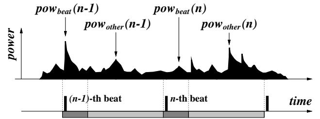
Fig. 16. Finding the local maximum of the power.
