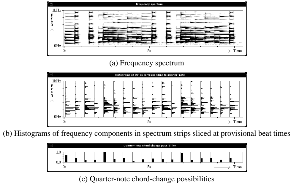
Fig. 6. Example of obtaining a chord-change possibility on the basis of provisional beat times.
