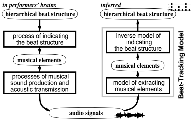
Fig. 3. Beat-tracking model.
