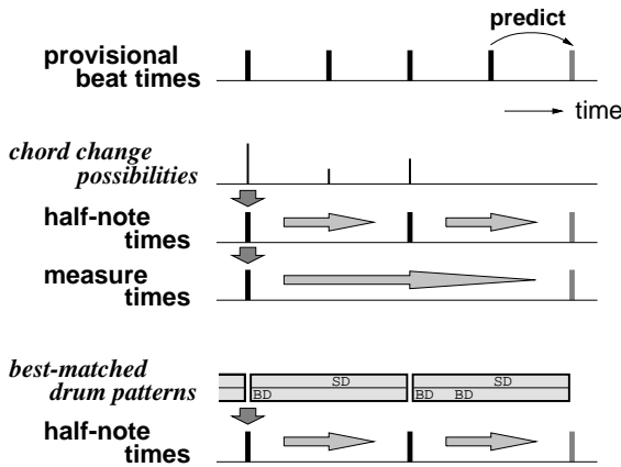
Fig. 10. Knowledge-based inferring.
