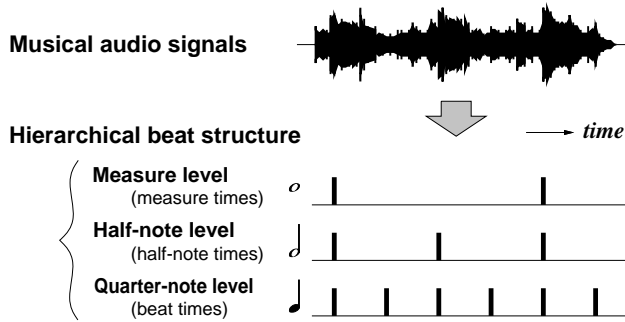
Fig. 1. Beat-tracking problem.
