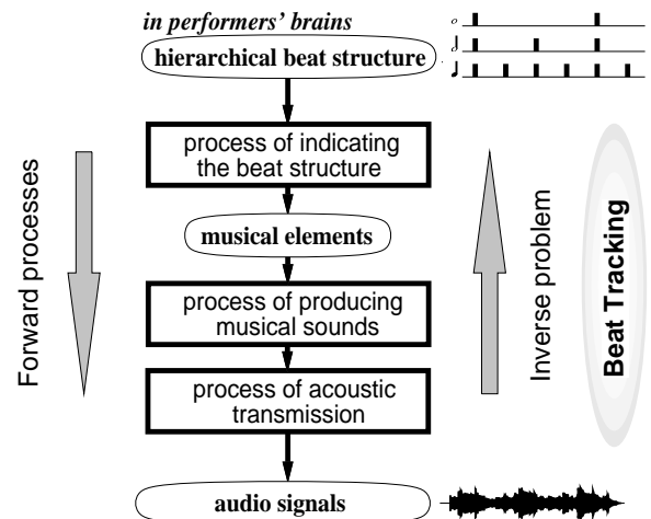
Fig. 2. Beat tracking as an inverse problem.
