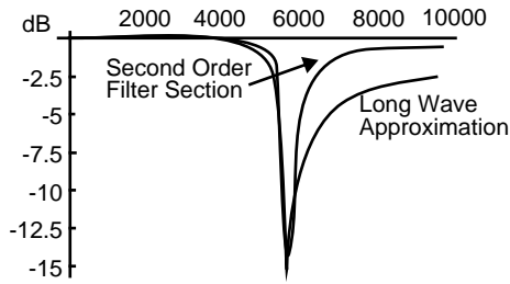
Fig. 3- The frequency response of a small section of a long wave model of the BM is compared to an approximation based on a second order filter. A large number of these sections are combined to form the overall lowpass filter characteristic of the cochlea.
