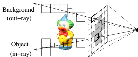
Fig. 4.2 Pixel-rays.
