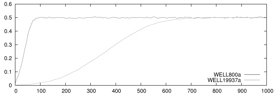
Fig. 5. \gamma_{n,5} for the WELL800a (top line) and WELL19937a (lower line).
