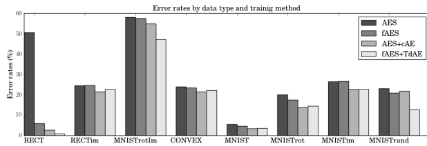
Figure 4. Error rates with and without pre-training, using ordinary and factored class-specific autoencoders.
