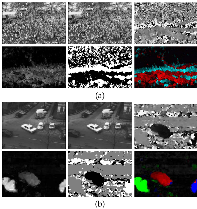
Fig. 6. Thresholding of optical flow data. (a) pilgrims sequence: two frames, angle and magnitude of flow vectors, two classes after thresholding, flow vector magnitudes colour coded according to class. (b) Hamburg taxi sequence: two frames, angle and magnitude of flow vectors, three classes after thresholding, flow vector magnitudes colour coded according to class.
