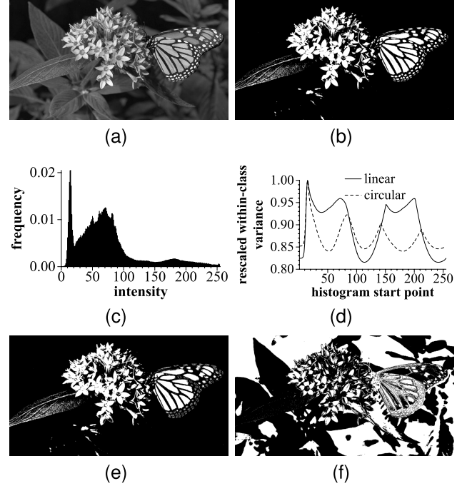
Fig. 5. An example of an image in which the thresholds selected by the algorithms using the linear (e) and circular (f) statistics produce an unusually large difference. The result using the standard (non circular histogram) Otsu criterion is shown in (b). The image's intensity histogram is shown in (c), and the within class variances as a function of threshold location are shown in (d).
