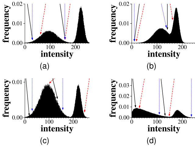
Fig. 2. Various synthetic distributions (a-d four typical histograms and corresponding thresholding results) showing the circular thresholds selected according to different criteria. The solid line corresponds to any of the following: \frac{\sigma_B^2}{\sigma_W^2} , \frac{\sigma_T^2}{\sigma_W^2} , \frac{\sigma_B^2}{\sigma_T^2} ; red dashed line: \sigma_B^2 ; blue dotted line: \sigma_W^2 .
