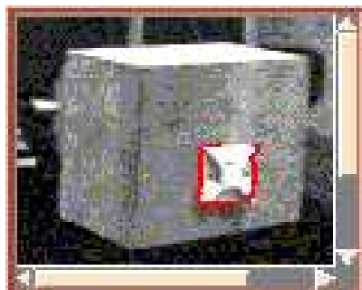
Convergence
