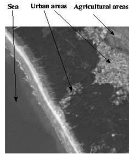
Texture
