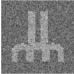
NdG
